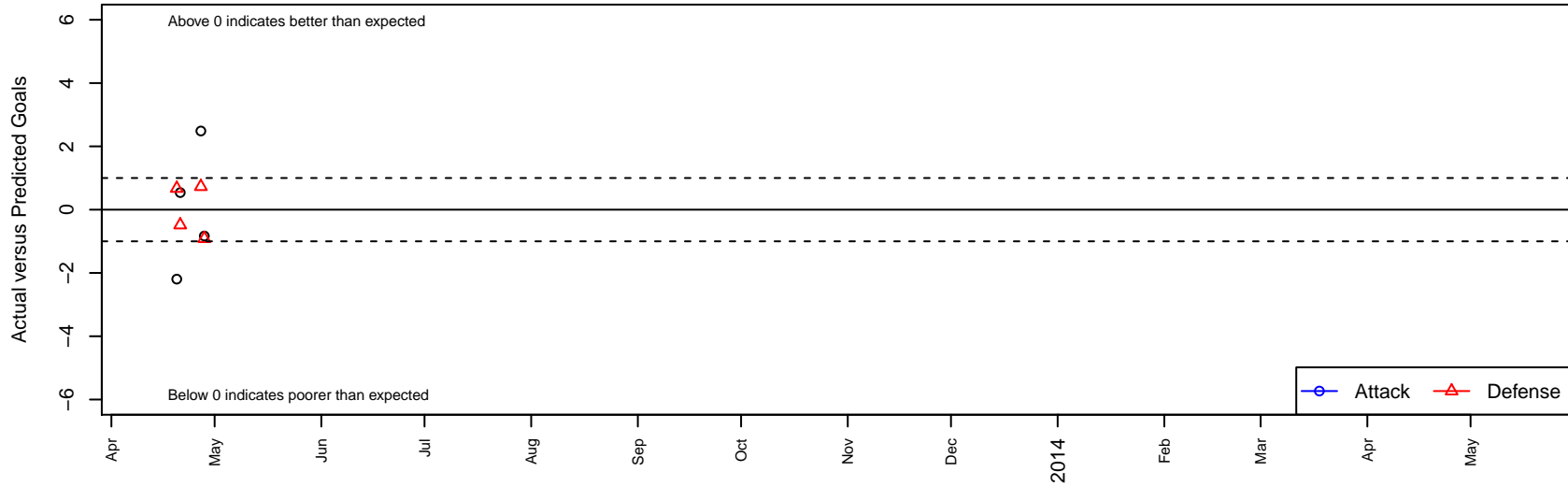
HSC Chivas B95 Dots are actual minus expected GF (blue circles) and GA (red triangles). Blue line is smoothed change in attack strength. Red is smoothed change in defense strength.
